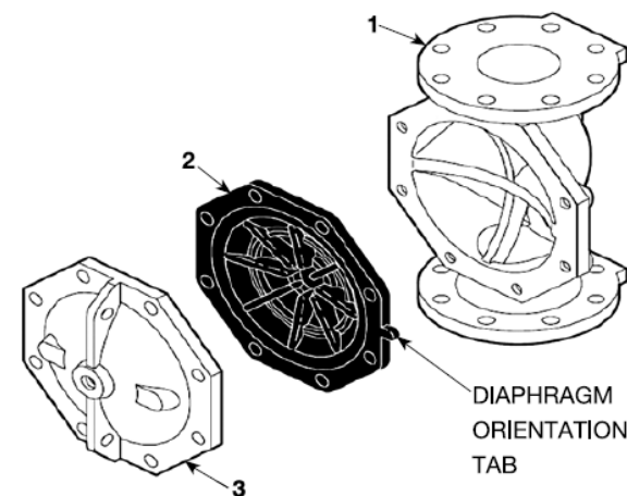
1. Valve Body 2. Elastomeric diaphragm 3. Valve Cover Plate
